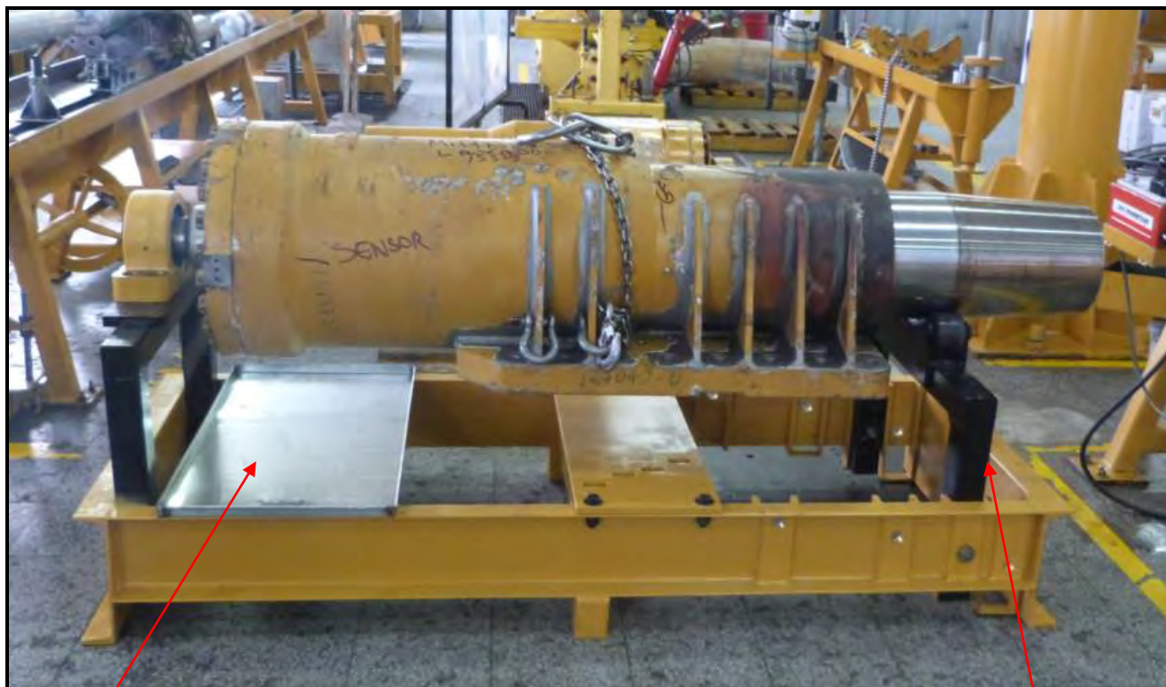
Photo 1: Suspension Cylinder Stand
