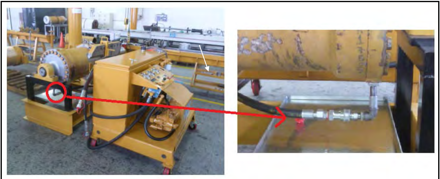
Photo 5. Fill with oil
